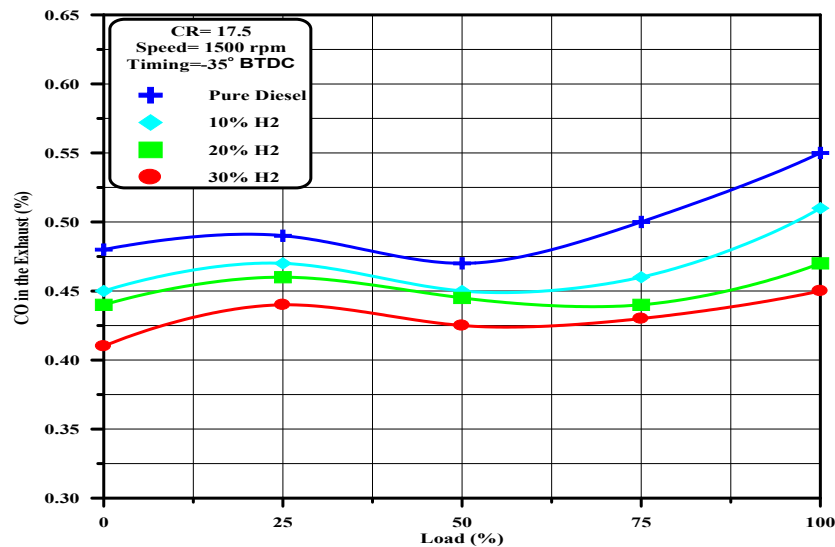
Fig 11 Variation of Carbon Monoxide with Load for Different Hydrogen Blending Ratios
