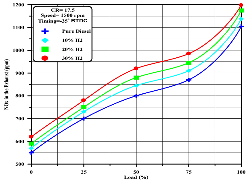
Fig 14 Variation of \text{NO}_x with Load for Different Hydrogen Blending Ratios
